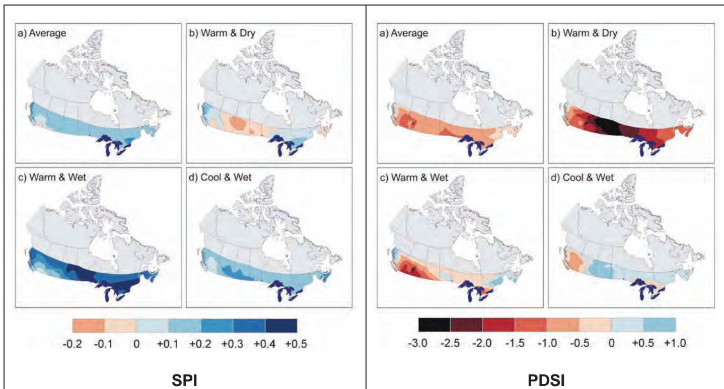
Figure 2: Projected average changes in SPI and PDSI values over southern Canada based on a) average, b) warm and dry, c) warm and wet, and d) cool and wet climate-change scenarios. The scenarios are based upon 30-year projected changes in temperature and precipitation for the period 2041-2070 (relative to the 1961-1990 baseline) using the A2 and B2 emission scenarios from multiple GCMs. Maps provide agricultural year (September to August) SPI and PDSI changes (from Bonsal and Regier, 2006).
